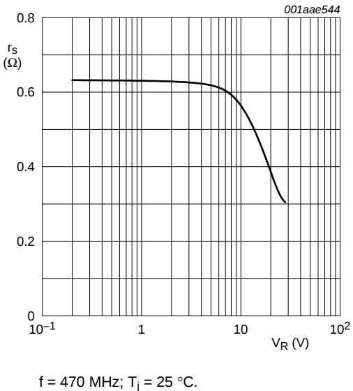
Fig 3. Diode series resistance as a function of reverse voltage; typical values
